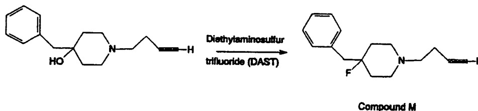
Scheme 13
